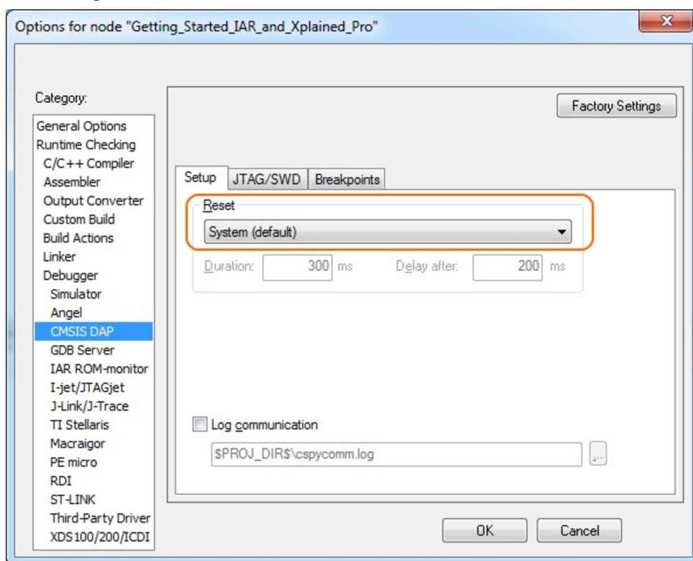
Figure 4-4. Configure Reset
