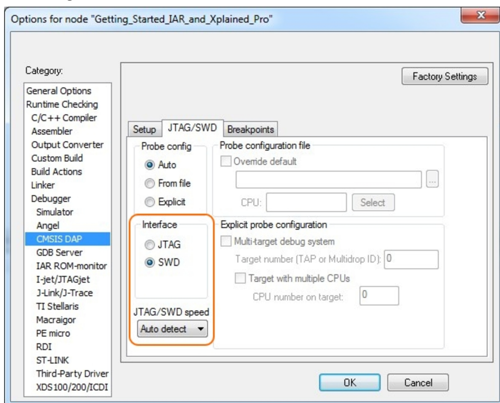
Figure 4-5. Configure Interface
