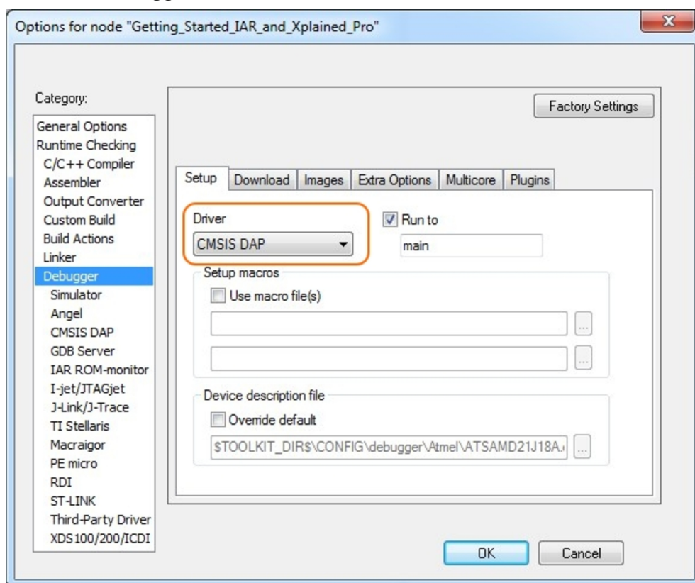
Figure 4-2. Select Debugger
