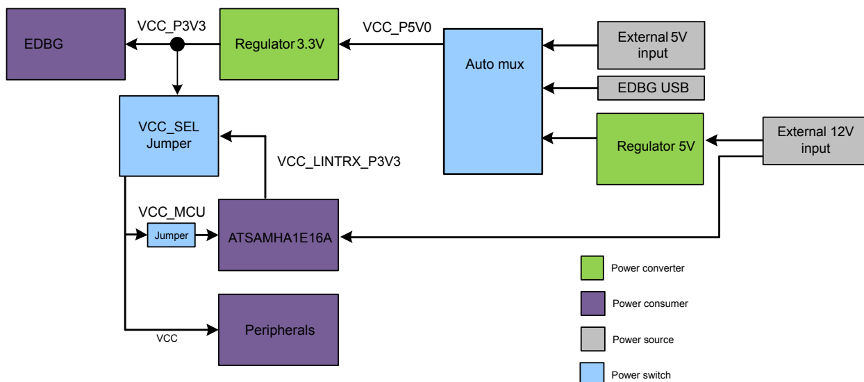
Figure 3-1. Power Supply Block Diagram
