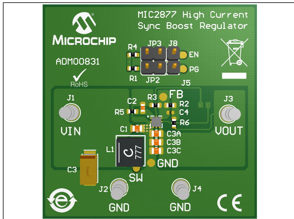
FIGURE 1-1: MIC2877 Evaluation Board Top View.
