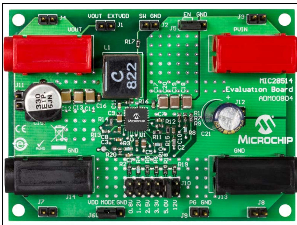
FIGURE 1-1: MIC28514 Evaluation Board.
