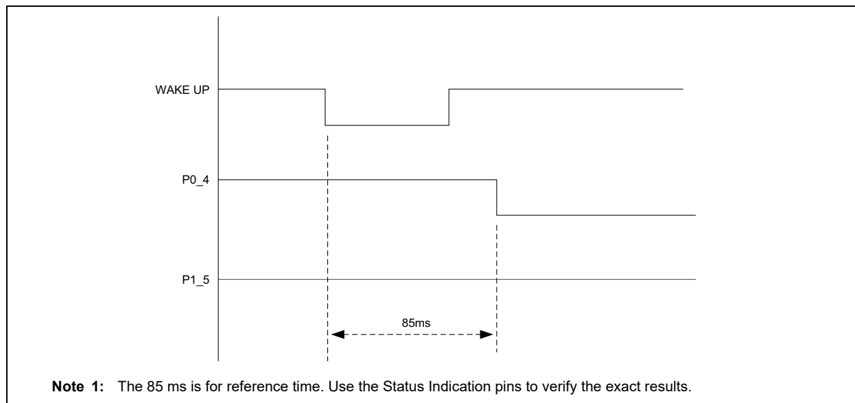
FIGURE 2-5: WAKE-UP TIME (1)
