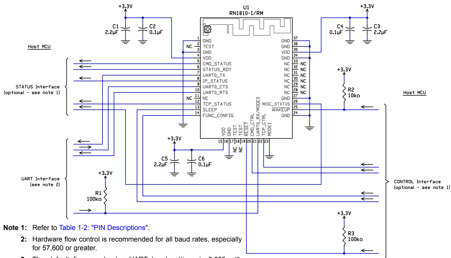
FIGURE 3-1: APPLICATION SCHEMATIC
