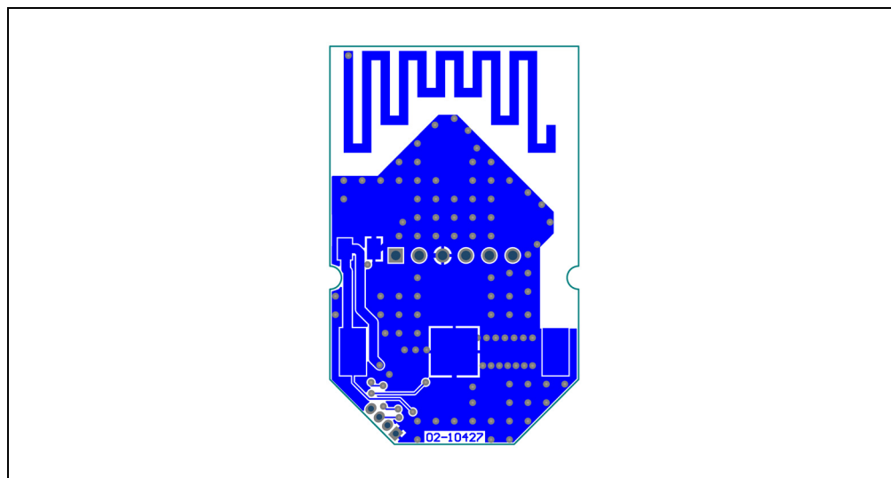
FIGURE A-4: KEY FOB PCB ASSEMBLY - BOTTOM COPPER
