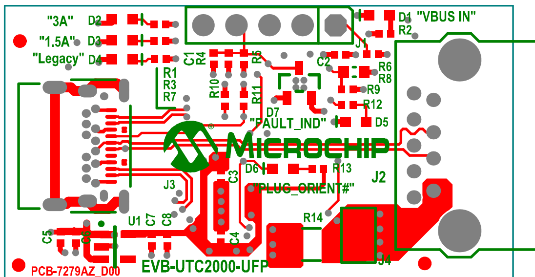
FIGURE C-2: EVB-UTC2000-UFP TOP AND BOTTOM SILK SCREEN IMAGES
