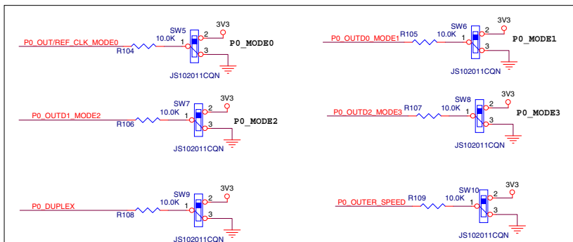
FIGURE B-7: EVB-LAN9355 EVALUATION BOARD SCHEMATIC 7
