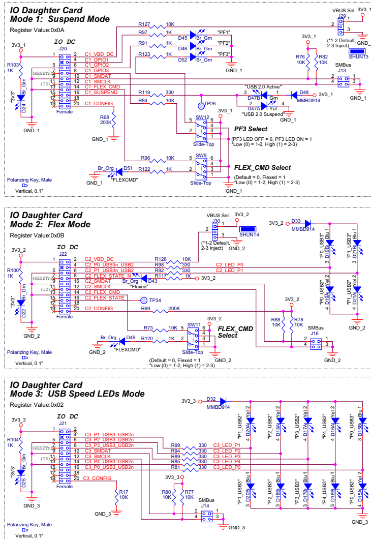
FIGURE B-1: EVB-USB5734 EVALUATION BOARD SCHEMATIC 3
