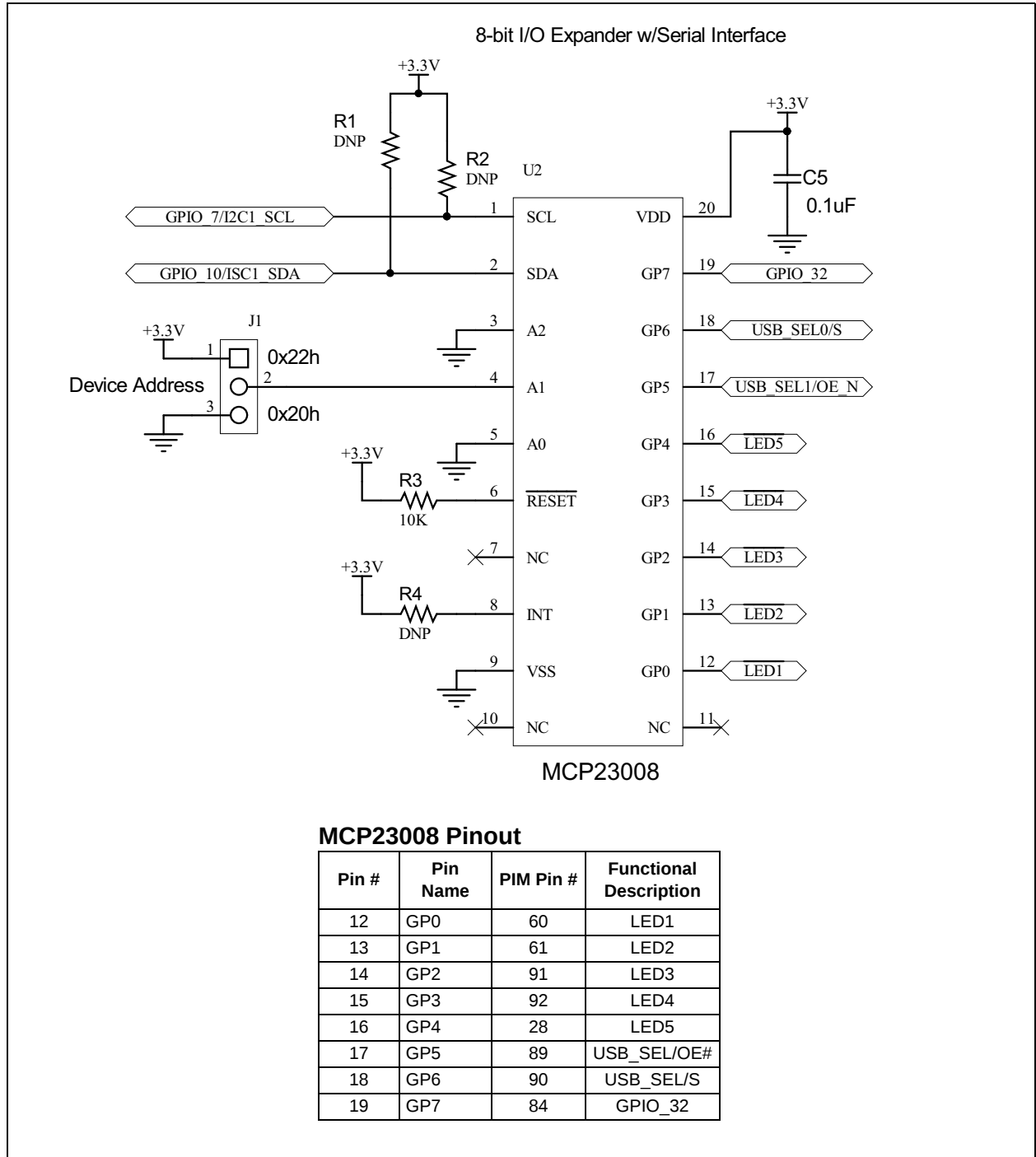
FIGURE 3: MCP23008 EXPANDER
