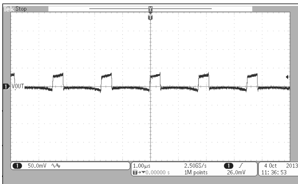
FIGURE C-3: Output Voltage Ripple/Noise ( V_{IN} = 24V , I_{OUT} = 4A , BW = 20\text{ MHz} ).
