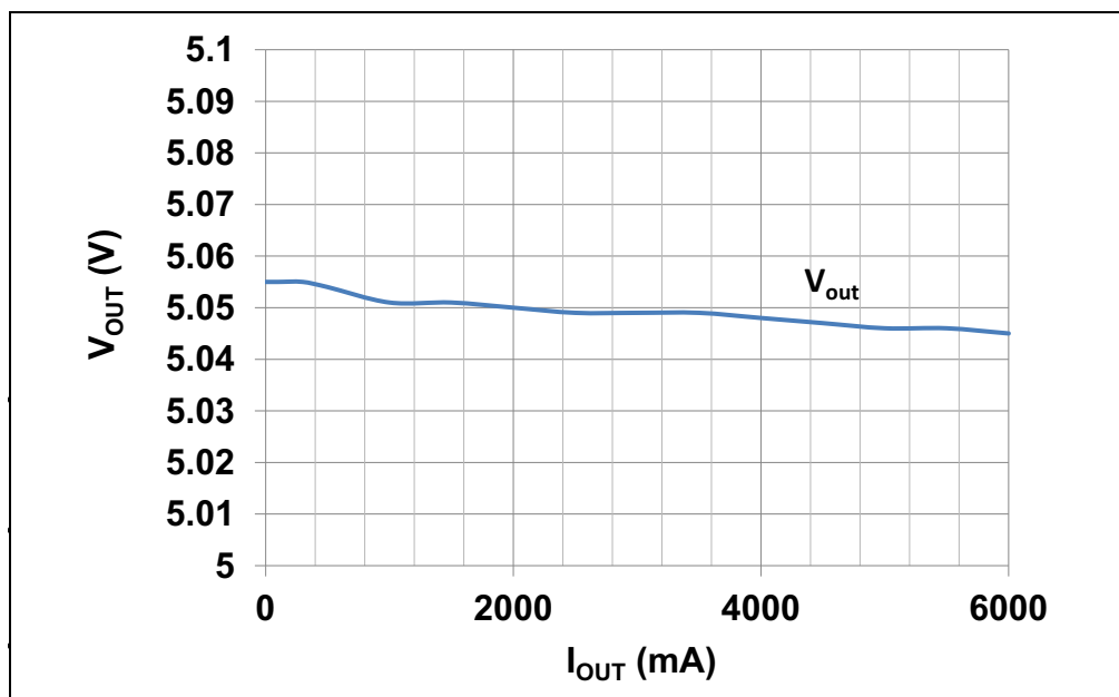
FIGURE C-2: Load Regulation ( V_{IN} = 24V ).
