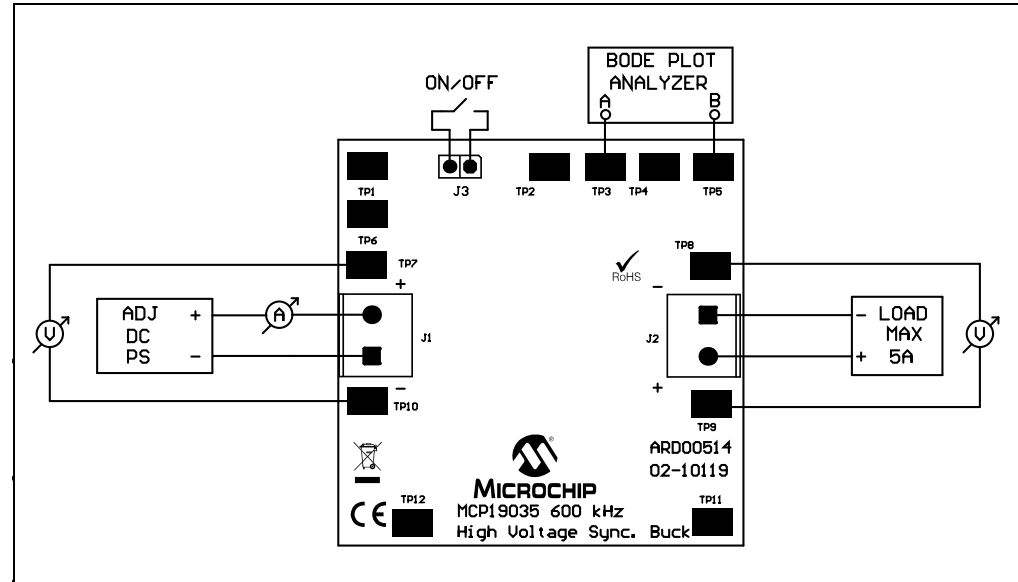
FIGURE 2-1: Typical Test Setup.
