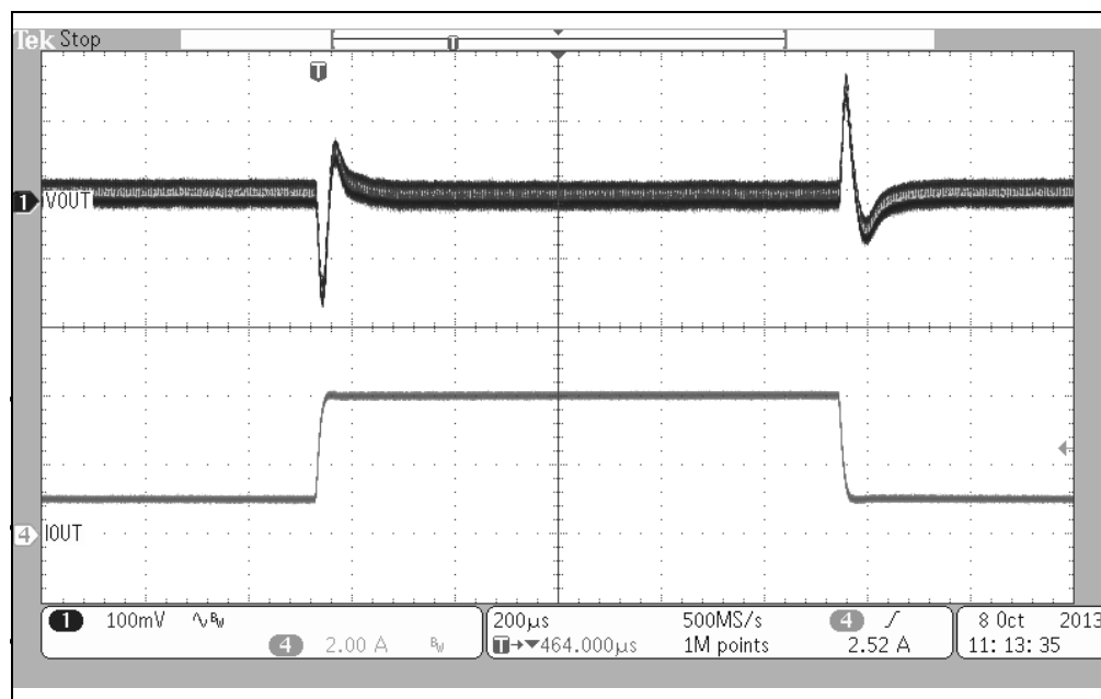
FIGURE C-5: Step Load ( V_{IN} = 24V ).
