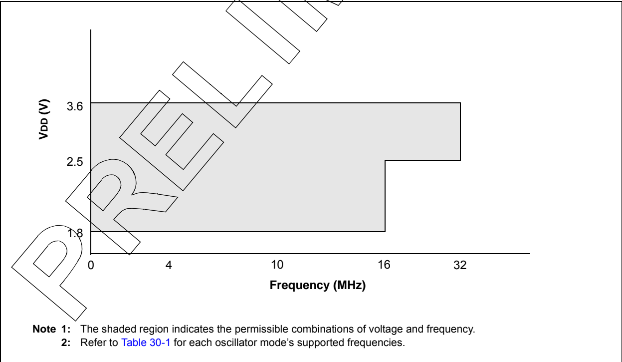
FIGURE 30-2: PIC16LF1847 VOLTAGE FREQUENCY GRAPH, -40°C ≤ TA ≤ +125°C
