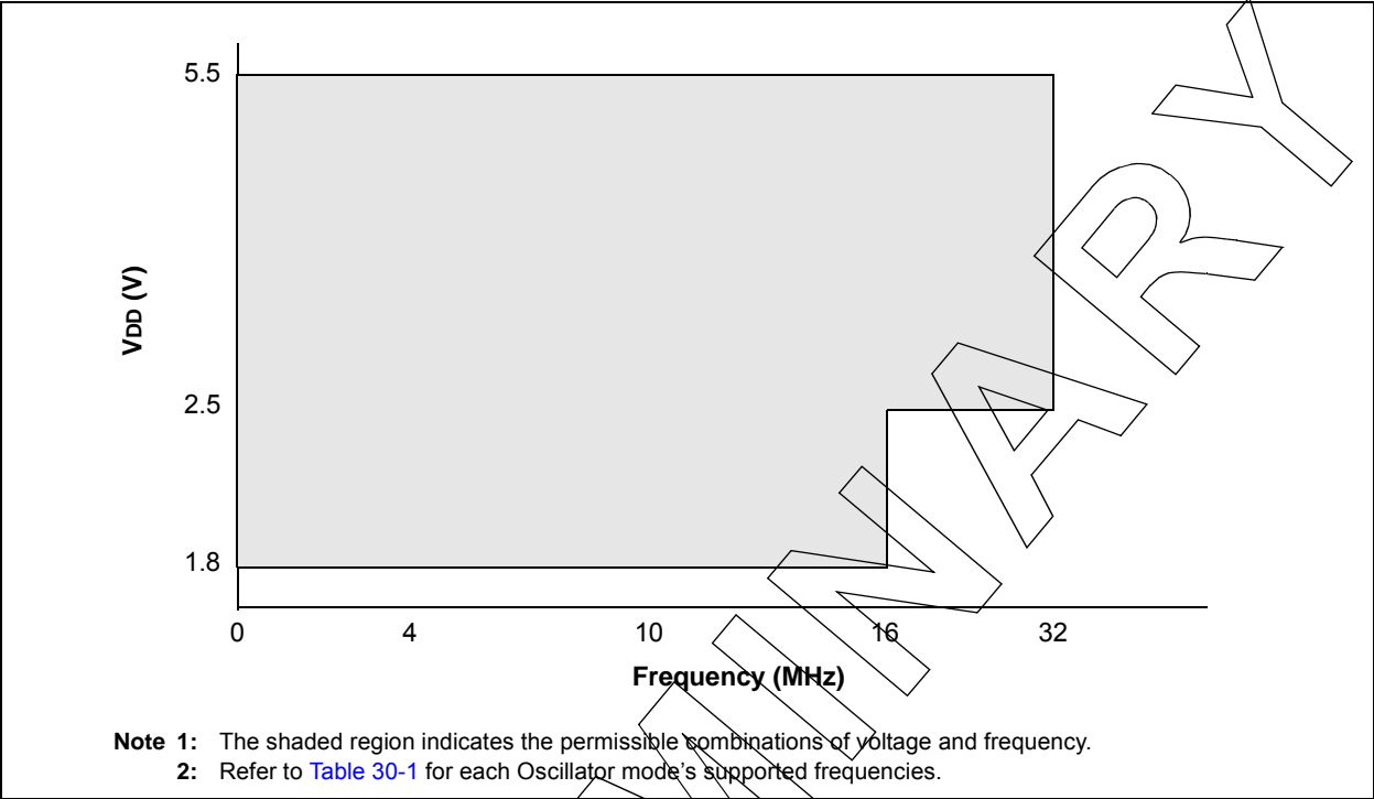
FIGURE 30-1: PIC16F1847 VOLTAGE FREQUENCY GRAPH, -40°C ≤ TA ≤ +125°C
