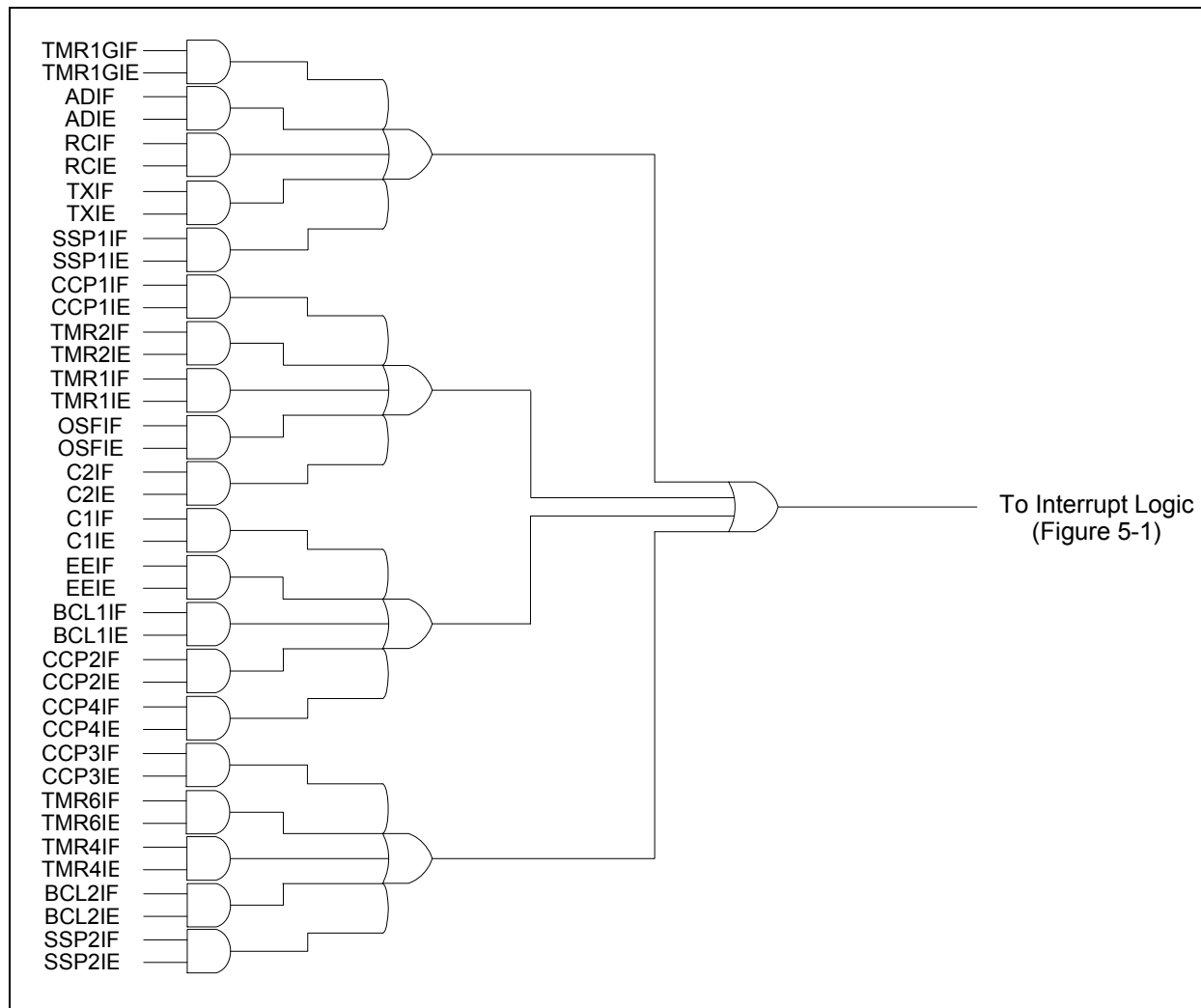
FIGURE 8-2: PERIPHERAL INTERRUPT LOGIC
