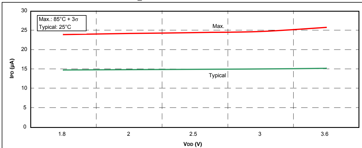
FIGURE 31-70: PIC16LF1937 FVR_DAC
