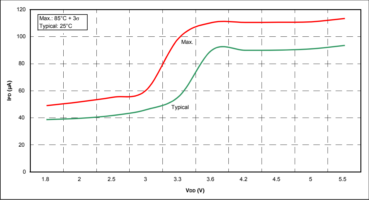
FIGURE 31-68: PIC16LF1937 WDT
