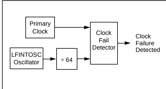
FIGURE 3-8: FSCM BLOCK DIAGRAM
