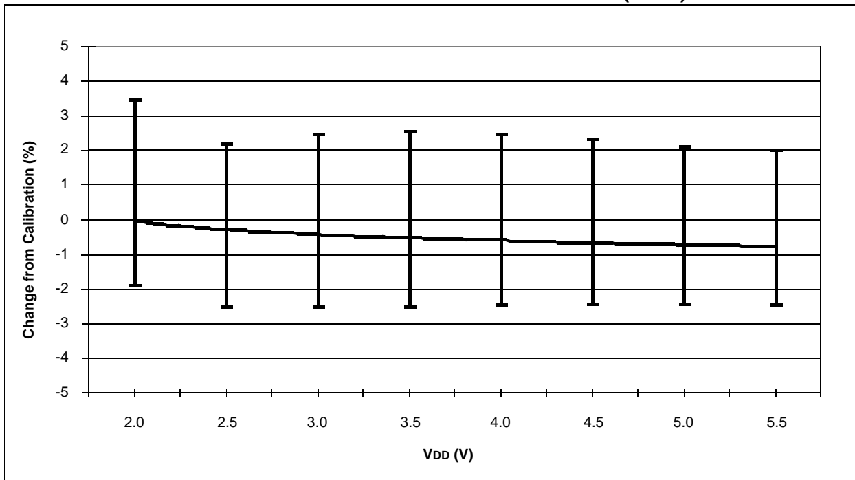
FIGURE 15-39: TYPICAL HFINTOSC FREQUENCY CHANGE vs. V_{DD} ( 125^{\circ}\text{C} )
