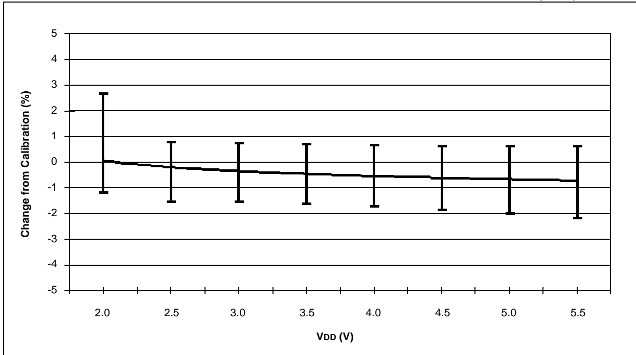
FIGURE 15-38: TYPICAL HFINTOSC FREQUENCY CHANGE OVER DEVICE V_{DD} ( 85^{\circ}\text{C} )
