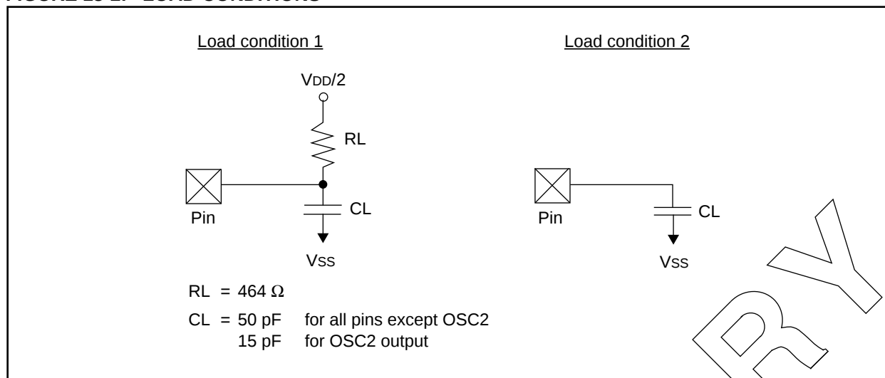
FIGURE 13-2: LOAD CONDITIONS
