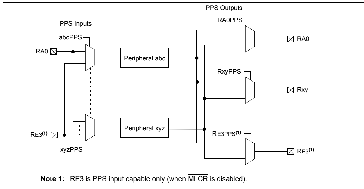
FIGURE 15-1: SIMPLIFIED PPS BLOCK DIAGRAM
