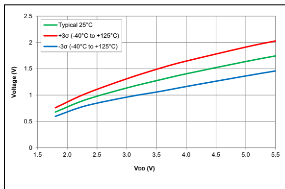
FIGURE 36-102: Schmitt Trigger Low Values
