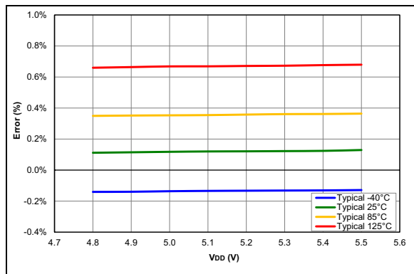
FIGURE 36-100: FVR Voltage Error 4x (PIC16F18326/46 only)
