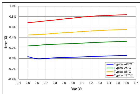
FIGURE 36-98: FVR Voltage Error 2x
