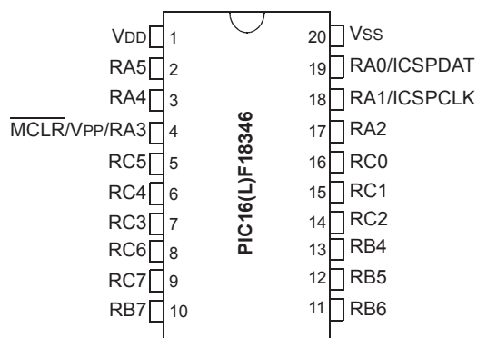
FIGURE 3: 20-PIN PDIP, SOIC, SSOP
