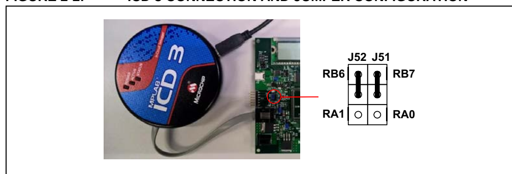
FIGURE 2-2: ICD 3 CONNECTION AND JUMPER CONFIGURATION
