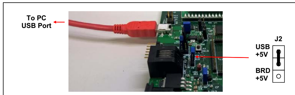
FIGURE 2-7: USB-POWERED BOARD CONFIGURATION
