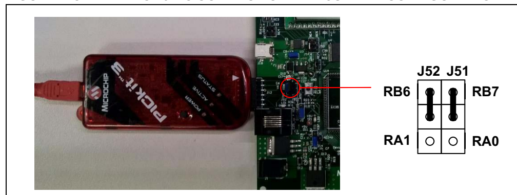
FIGURE 2-3: PICKit™ 3 CONNECTION AND JUMPER CONFIGURATION
