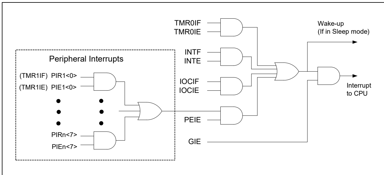
FIGURE 8-1: INTERRUPT LOGIC
