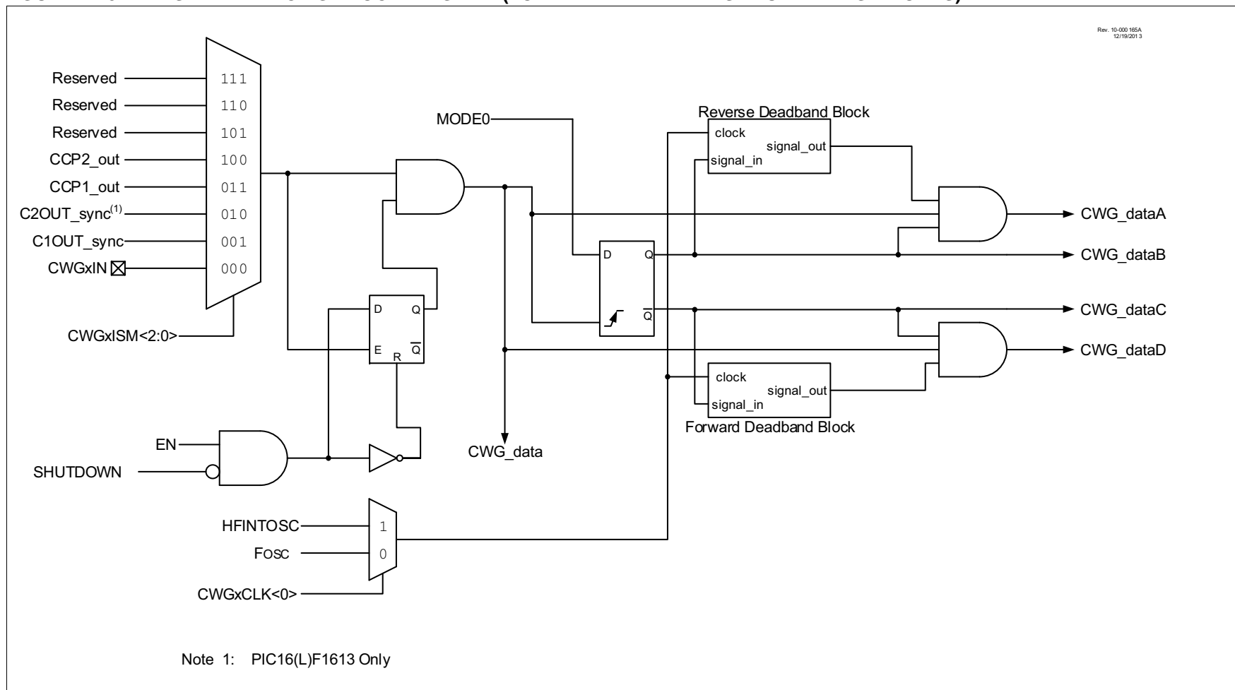
PIC12(L)F1612/16(L)F1613
