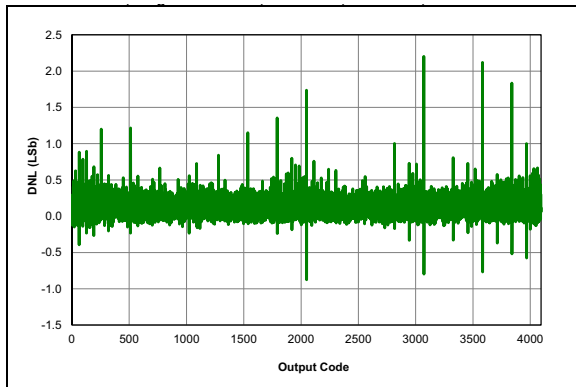
FIGURE 32-93: ADC 12-bit Mode, Single-Ended DNL, V_{DD} = 5.5V , T_{AD} = 1\text{ }\mu\text{S} , 25^\circ\text{C} .
