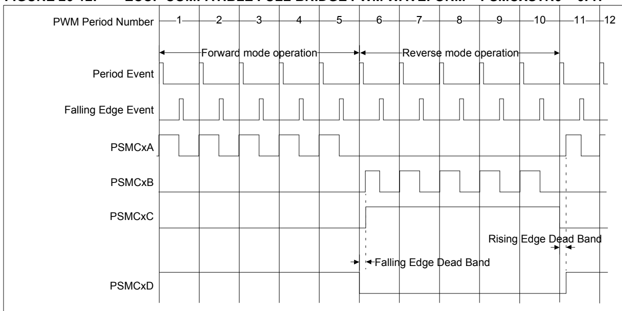
FIGURE 26-12: ECCP COMPATIBLE FULL-BRIDGE PWM WAVEFORM – PSMCXSTR0 = 0FH
