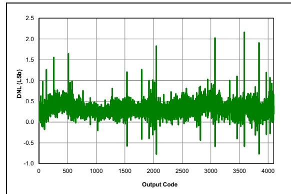
FIGURE 32-94: ADC 12-bit Mode, Single-Ended DNL, V_{DD} = 5.5V , T_{AD} = 4\text{ }\mu\text{S} , 25^\circ\text{C} .
