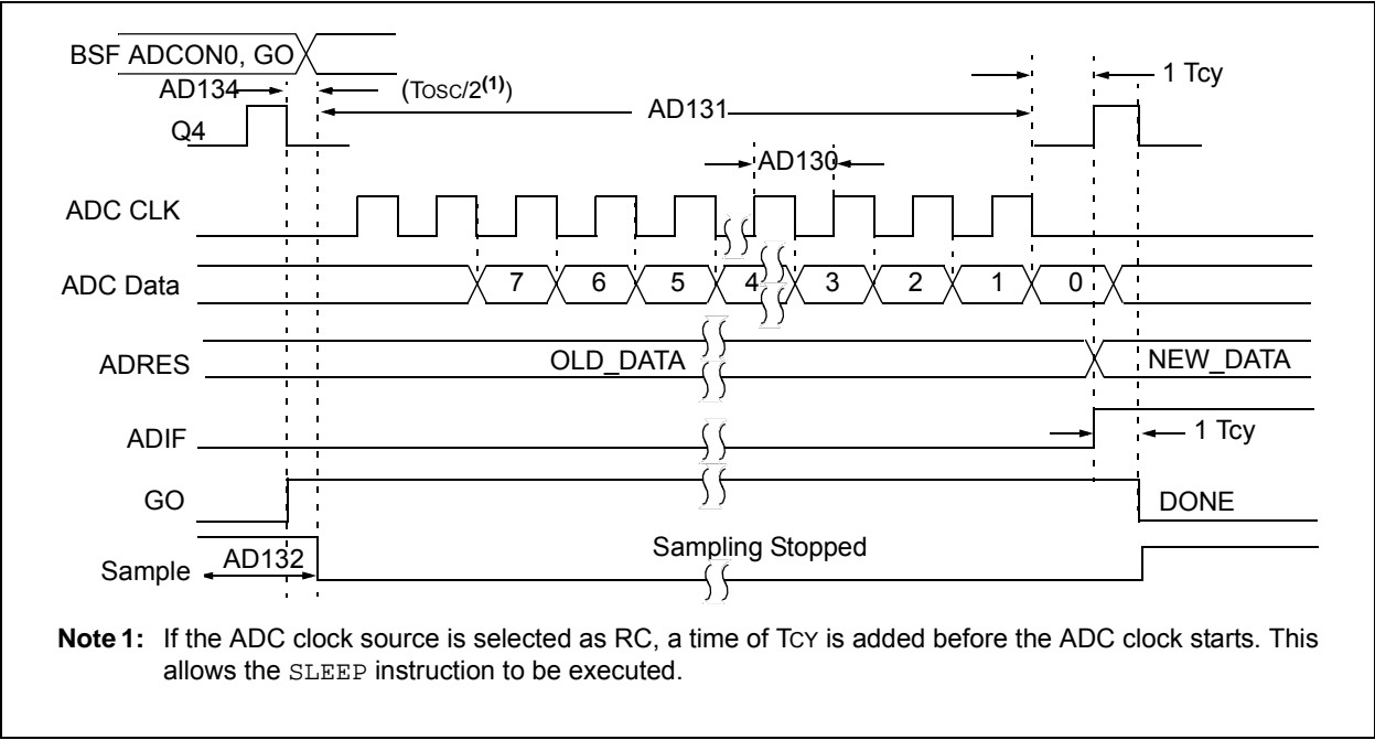
FIGURE 31-12: ADC CONVERSION TIMING (NORMAL MODE)
