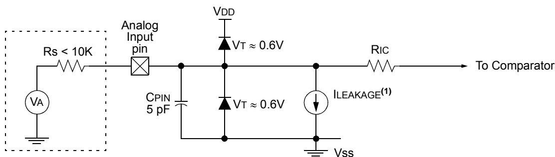
FIGURE 21-4: ANALOG INPUT MODEL
