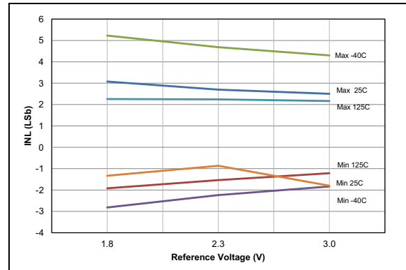
FIGURE 32-92: ADC 12-bit Mode, Single-Ended INL, V_{DD} = 3.0V , T_{AD} = 1\text{ }\mu\text{S} .
