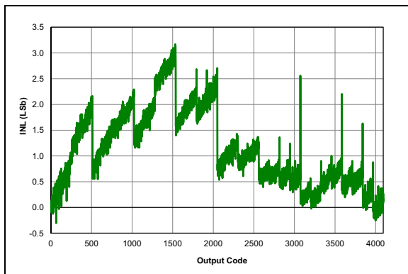
FIGURE 32-95: ADC 12-bit Mode, Single-Ended INL, V_{DD} = 5.5V , T_{AD} = 1\text{ }\mu\text{S} , 25^\circ\text{C} .
