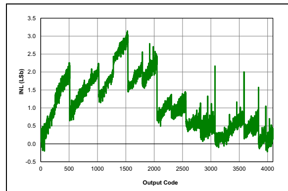
FIGURE 32-96: ADC 12-bit Mode, Single-Ended INL, V_{DD} = 5.5V , T_{AD} = 4\text{ }\mu\text{S} , 25^\circ\text{C} .
