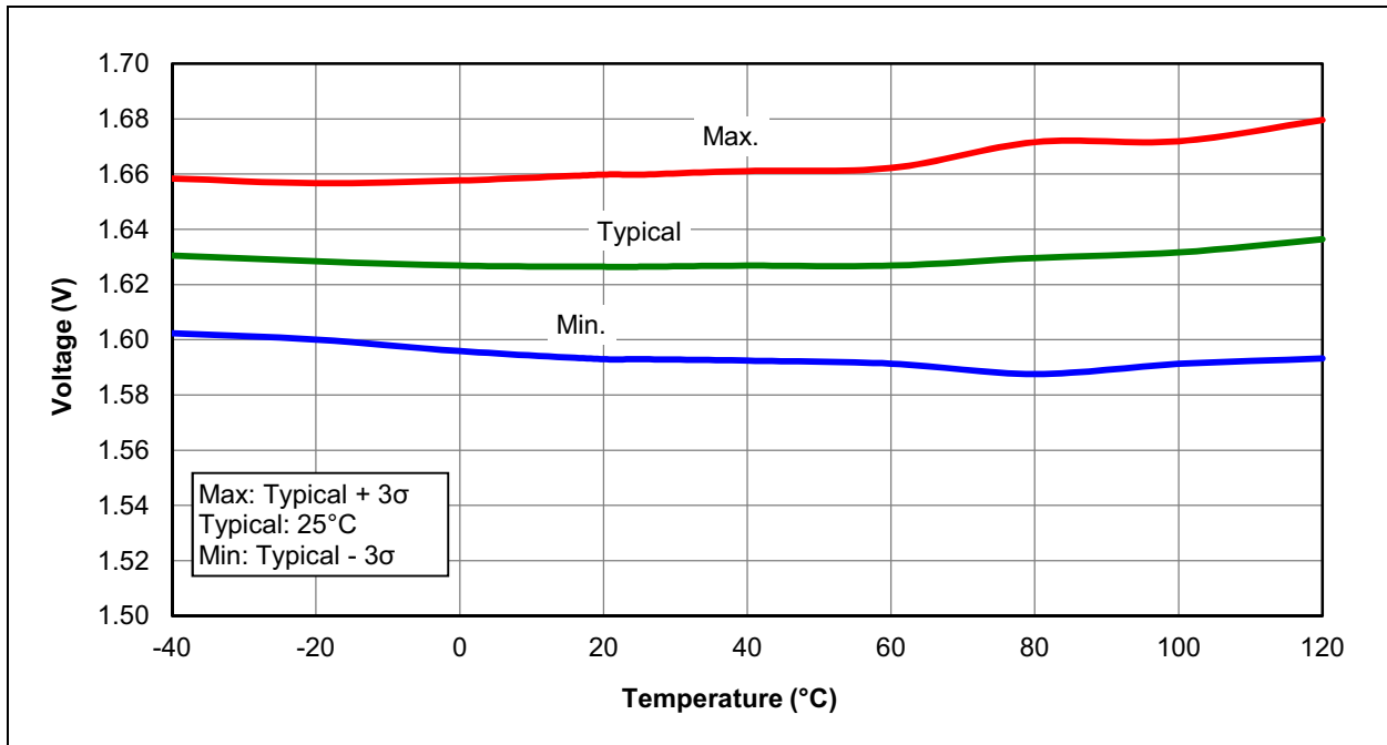
FIGURE 32-26: POR RELEASE VOLTAGE
