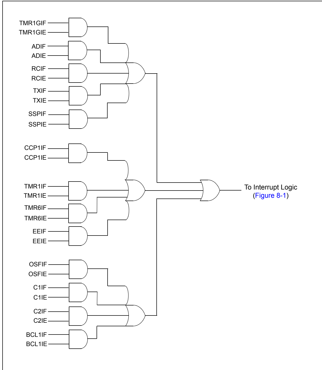
FIGURE 8-2: PERIPHERAL INTERRUPT LOGIC
