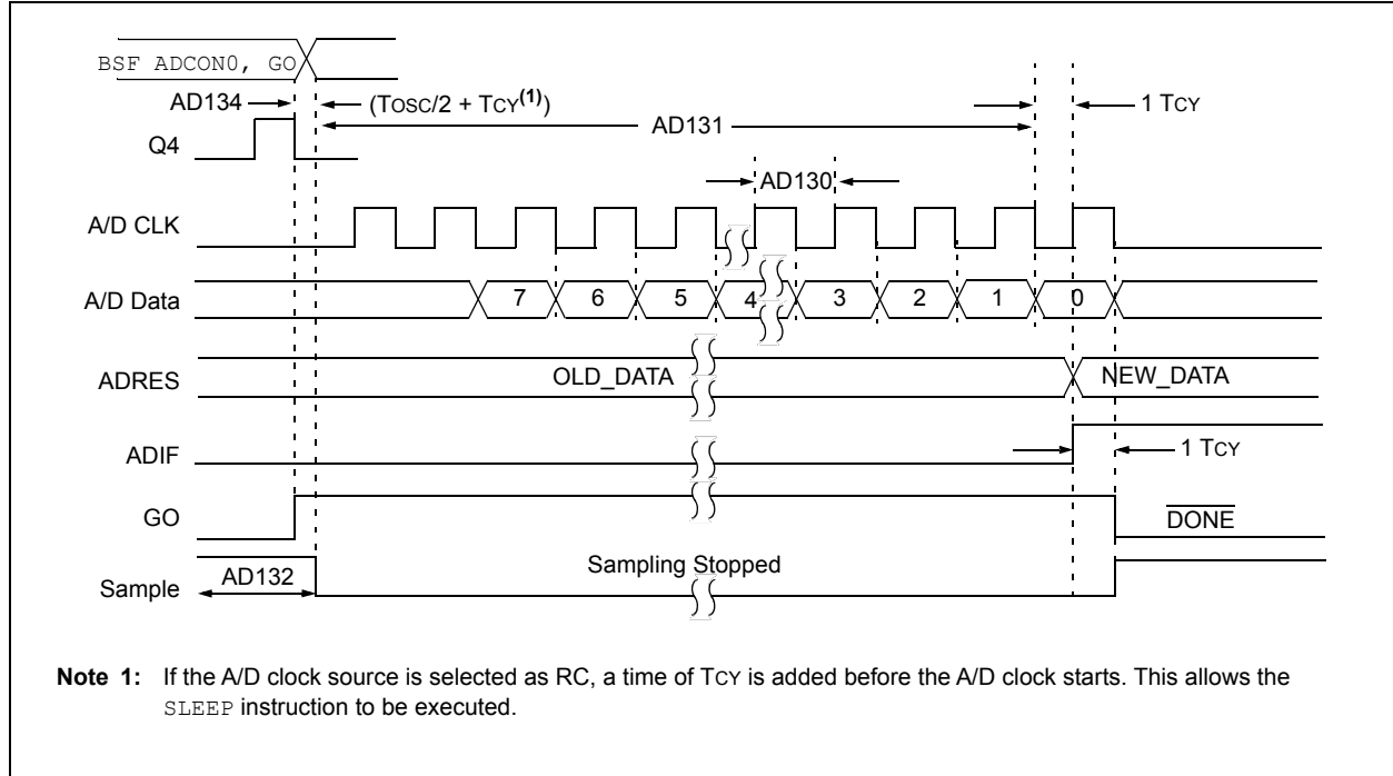
FIGURE 31-12: PIC16LF1824T39A A/D CONVERSION TIMING (SLEEP MODE)
