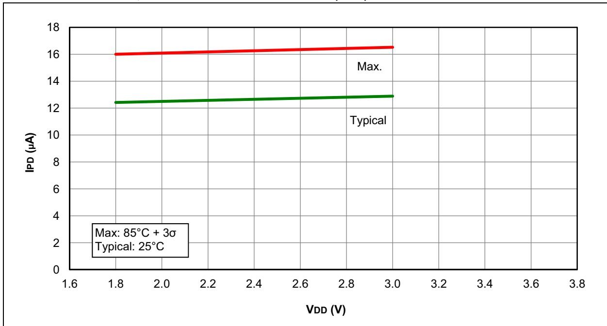
FIGURE 32-14: I_{PD} , FIXED VOLTAGE REFERENCE (FVR)
