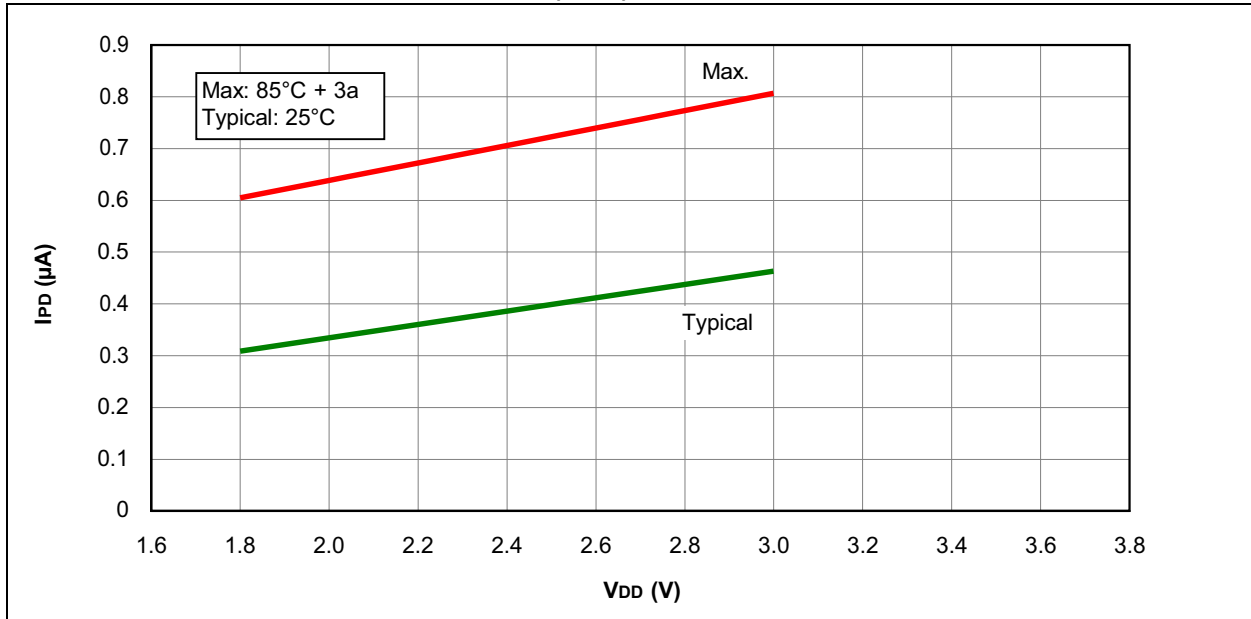
FIGURE 32-13: I_{PD} , WATCHDOG TIMER (WDT)
