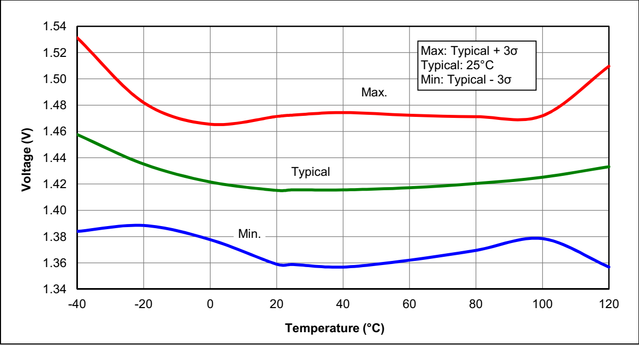
FIGURE 32-28: BROWN-OUT RESET VOLTAGE, BORV = 1
