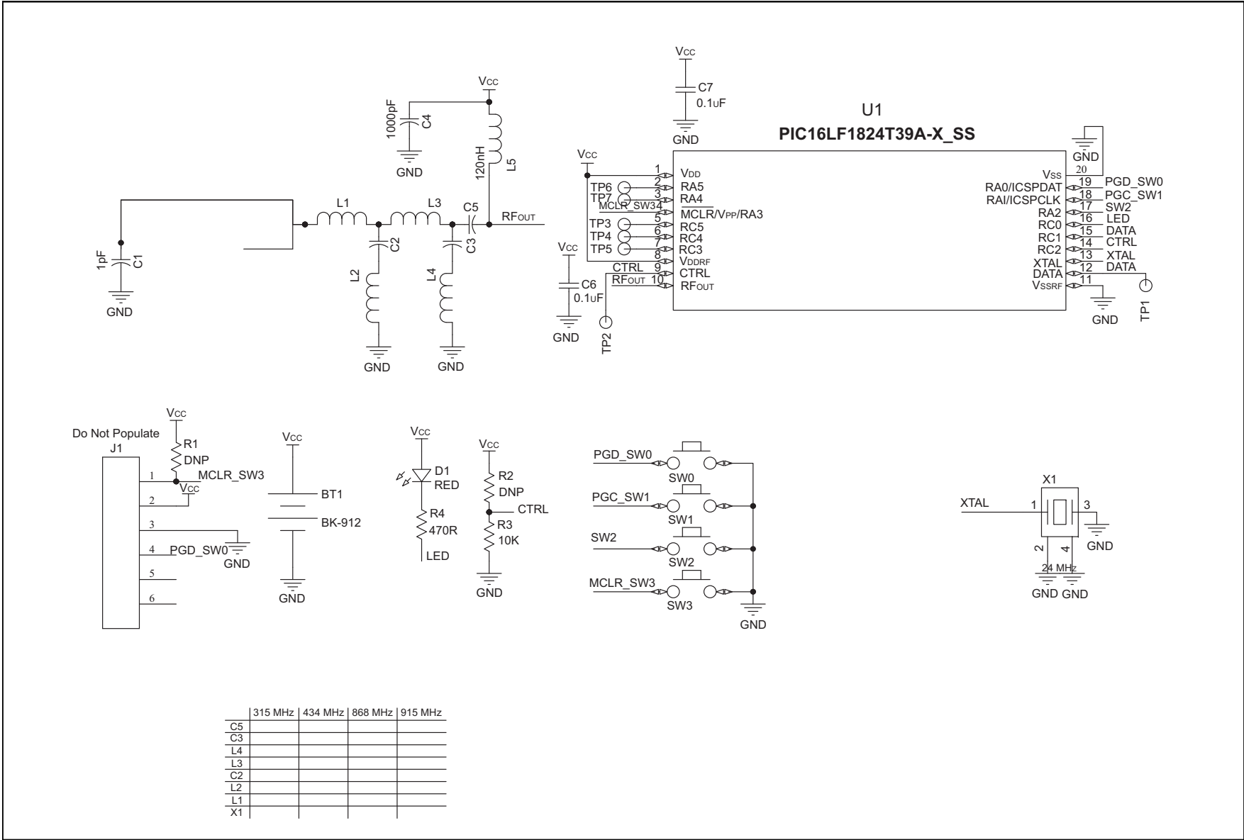
FIGURE 28-8: APPLICATION SCHEMATIC
