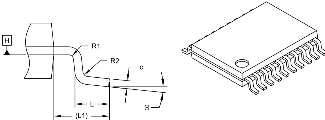
DETAIL B
