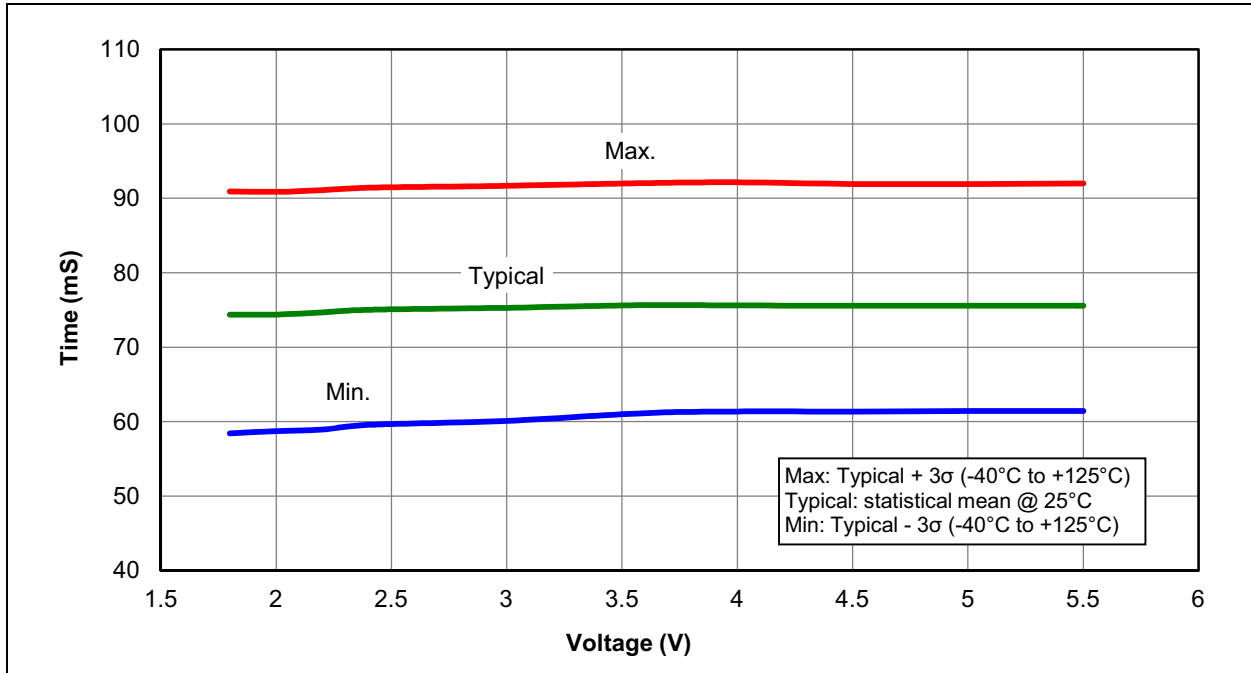
FIGURE 32-33: PWRT PERIOD
