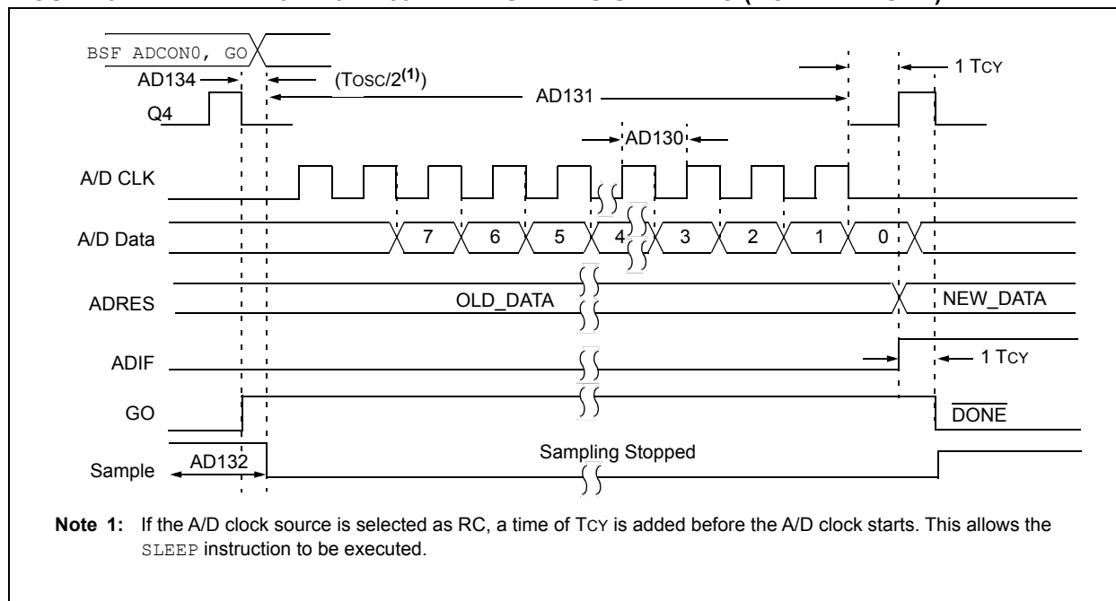
FIGURE 31-11: PIC16LF1824T39A A/D CONVERSION TIMING (NORMAL MODE)
