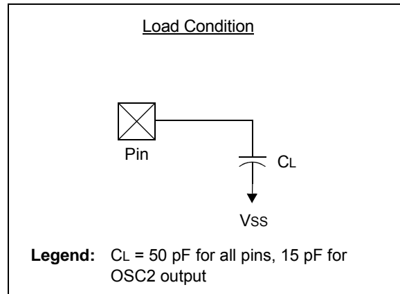
FIGURE 26-7: LOAD CONDITIONS
