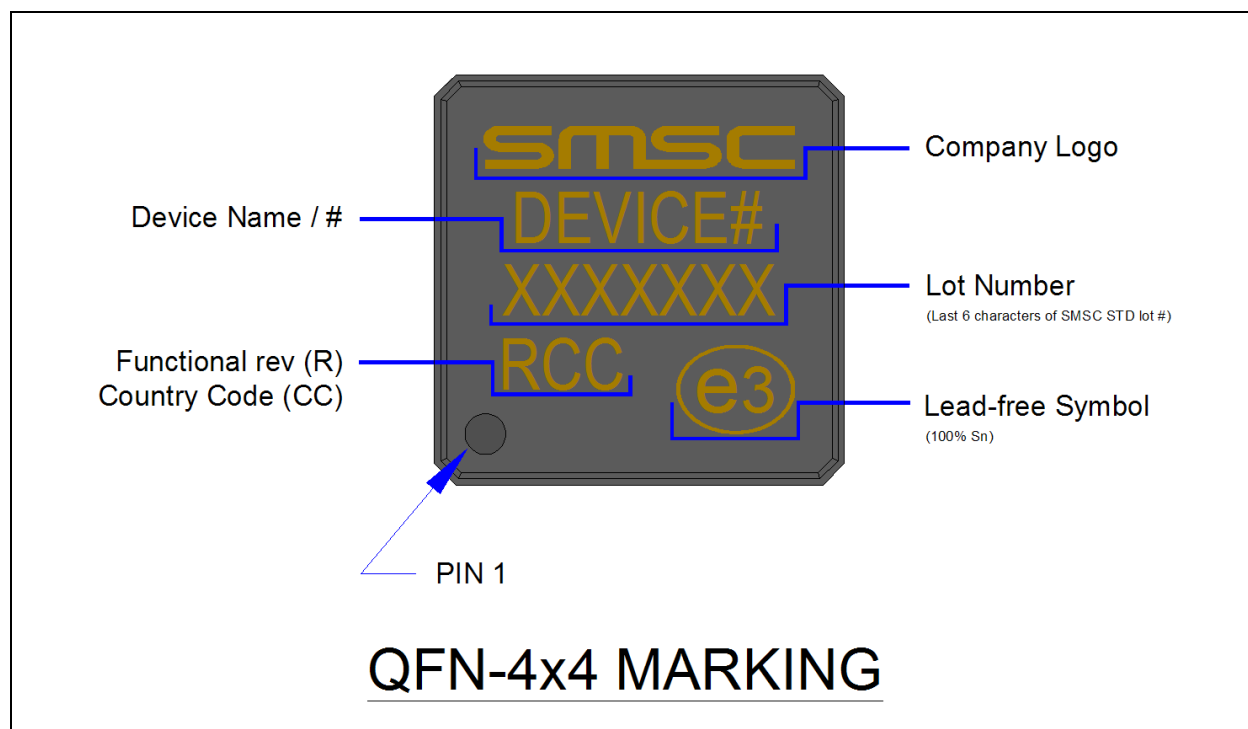
Figure 9.7 QFN, 4x4 Package Marking
