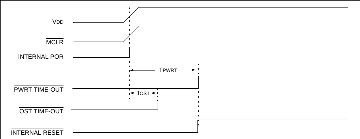
FIGURE 5-5: TIME-OUT SEQUENCE ON POWER-UP (MCLR TIED TO VDD)
