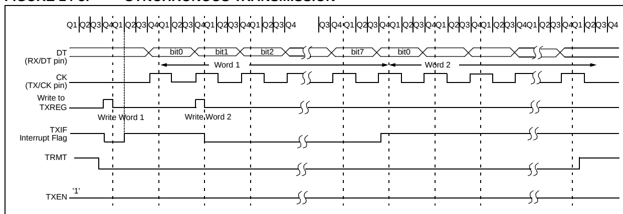
FIGURE 14-8: SYNCHRONOUS TRANSMISSION
