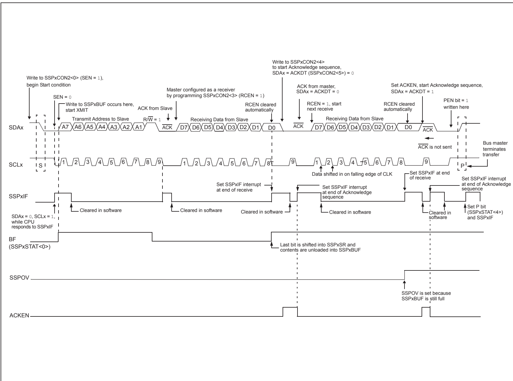
12 C MASTER MODE WAVEFORM (RECEPTION, 7-BIT ADDRESS)
