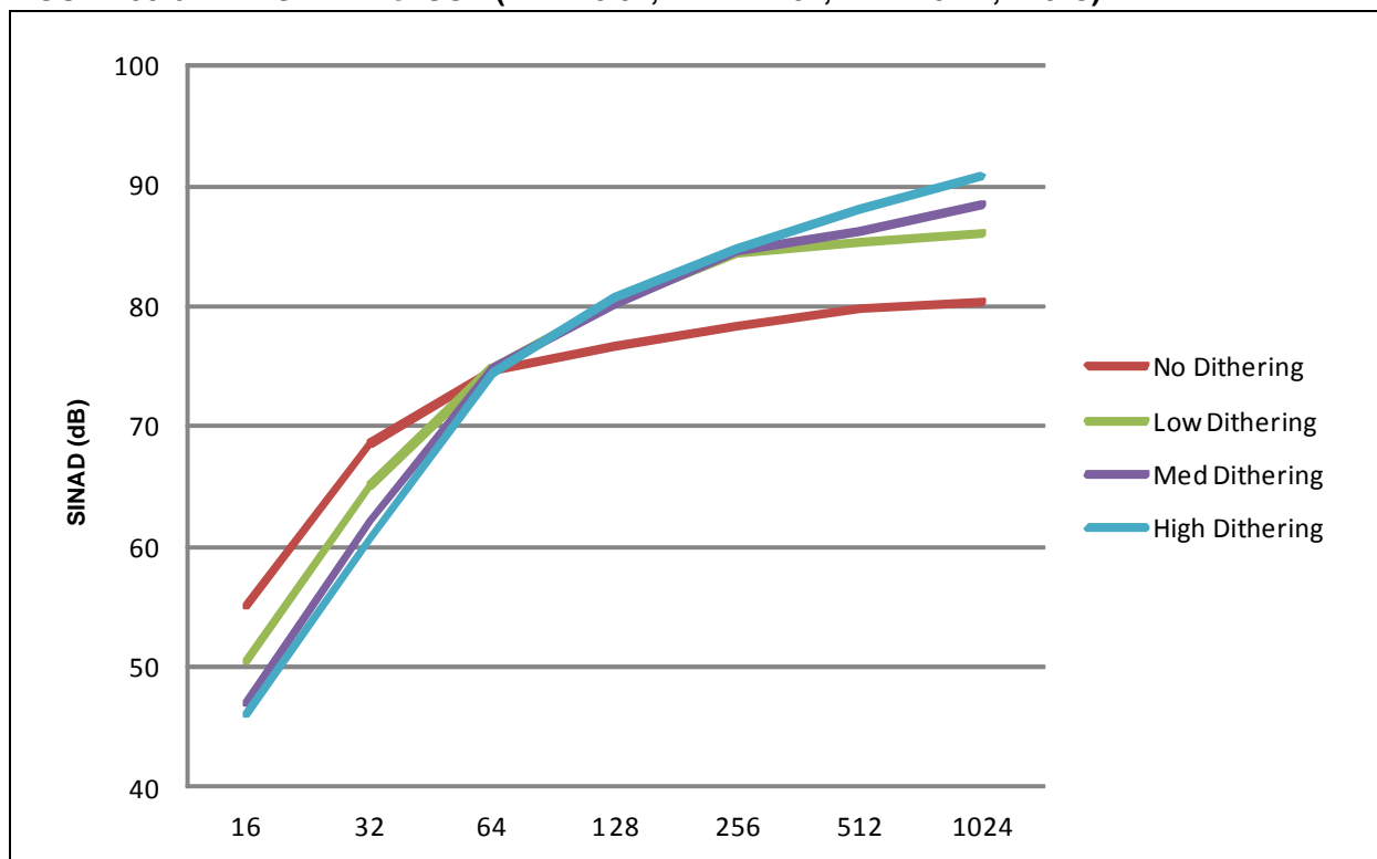
FIGURE 38-6: SINAD vs. OSR ( V_{DD} = 3.3V , V_{REF} = 2.0V , F_{IN} = 25 Hz, +25^{\circ}C )
