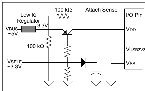
FIGURE 27-11: DUAL POWER WITH SELF-POWER DOMINANCE
