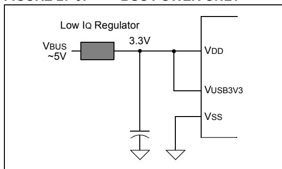
FIGURE 27-9: BUS POWER ONLY
