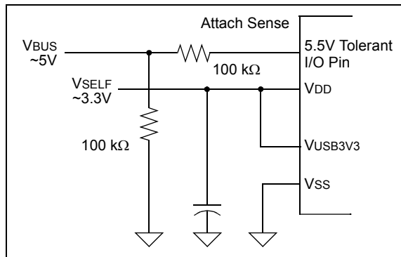
FIGURE 27-10: SELF-POWER ONLY
