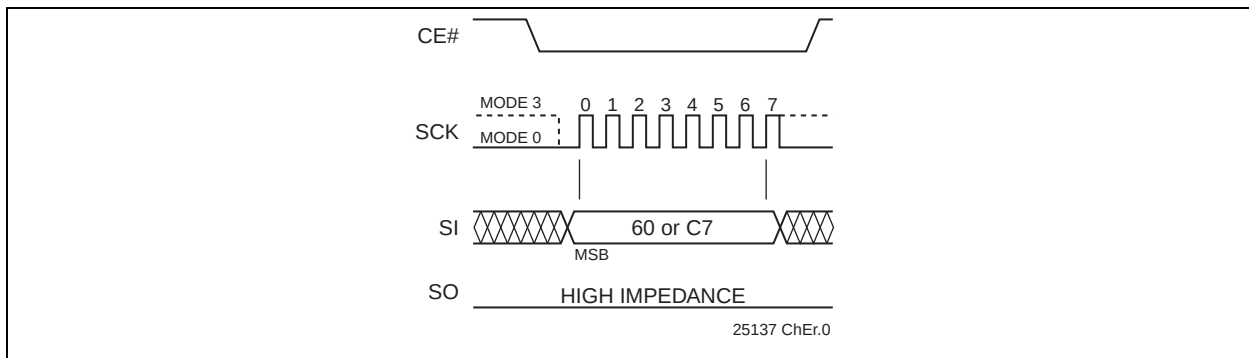
FIGURE 4-13: CHIP-ERASE SEQUENCE
