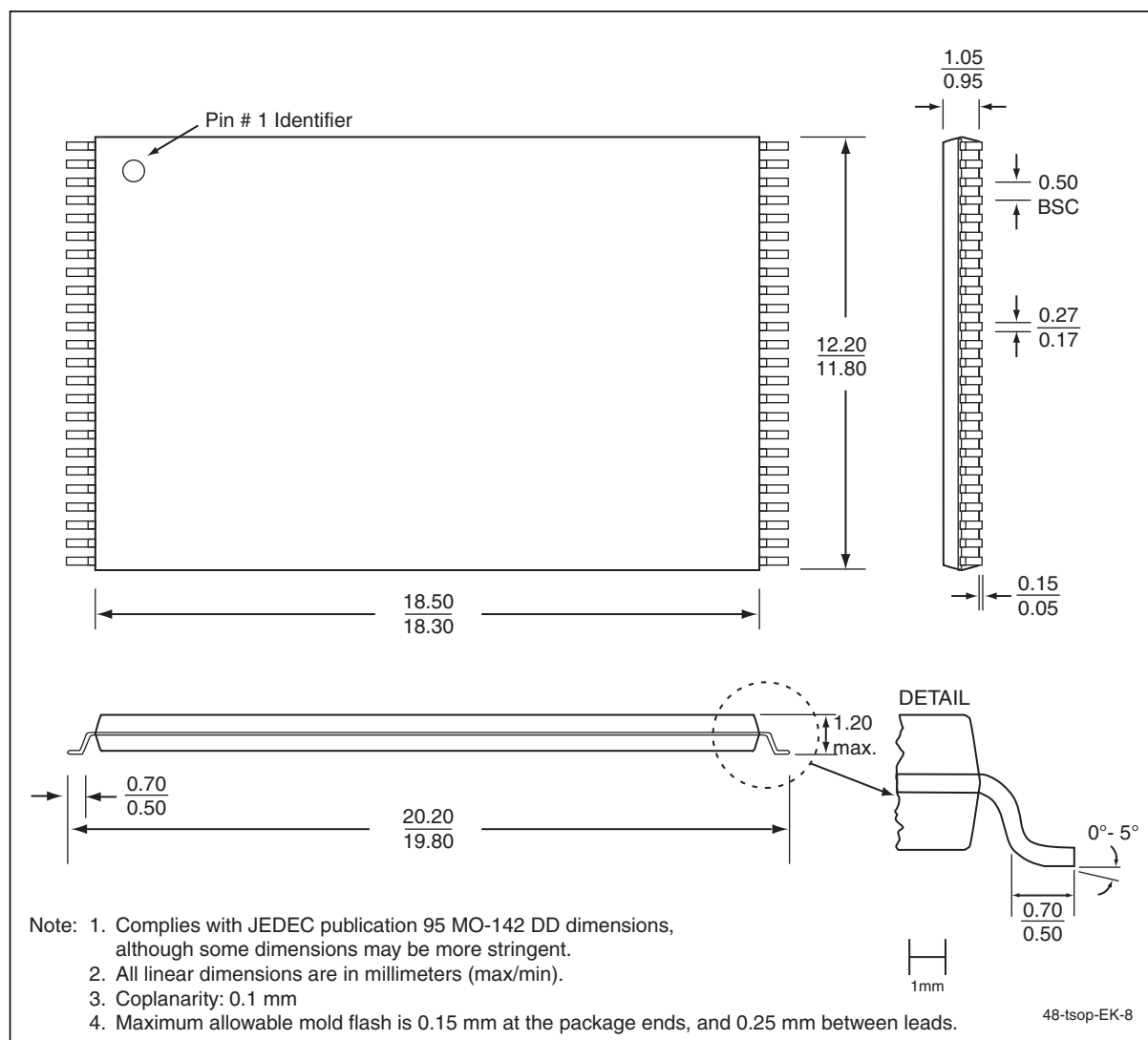
Figure 25: 48-lead Thin Small Outline Package (TSOP) 12mm x 20mm
