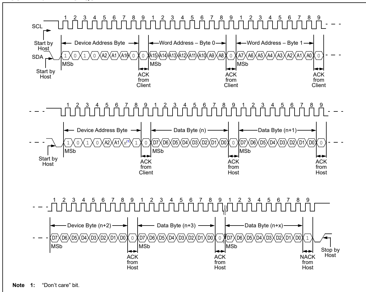
FIGURE 7-3: SEQUENTIAL READ
