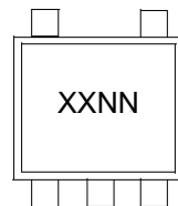
5-Lead SC-70
