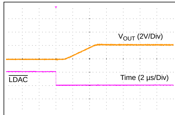
FIGURE 2-28: Full Scale Settling Time ( V_{REF} = \text{Internal} , V_{DD} = 5\text{V} , \text{UDAC} = 1 , Gain = x1, Code Change: 000h to FFFh).
