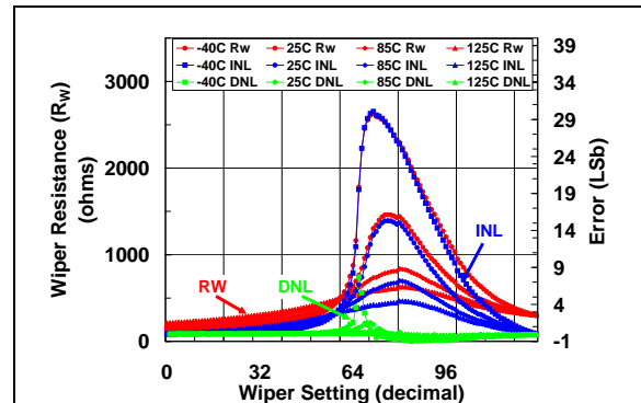
FIGURE 2-25: 10 k \Omega Rheo Mode : R_W ( \Omega ), INL (LSb), DNL (LSb) vs. Wiper Setting and Temperature ( V_{DD} = 2.7\text{V} ). ( I_W = 210\text{ }\mu\text{A} , B = V_{SS} ).
