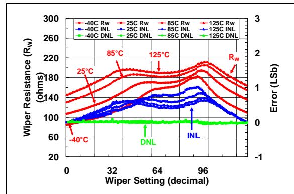
FIGURE 2-25: 10 k \Omega Rheo Mode : R_W ( \Omega ), INL (LSb), DNL (LSb) vs. Wiper Setting and Temperature ( V_{DD} = 2.7\text{V} ). ( I_W = 210\text{ }\mu\text{A} , B = V_{SS} ).
