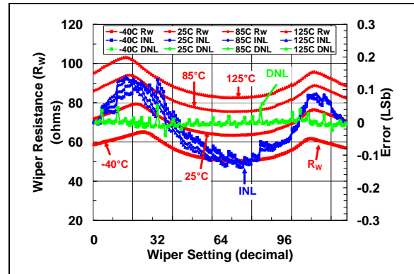
FIGURE 2-24: 10 k \Omega Rheo Mode : R_W ( \Omega ), INL (LSb), DNL (LSb) vs. Wiper Setting and Temperature ( V_{DD} = 5.5\text{V} ). ( I_W = 450\text{ }\mu\text{A} , B = V_{SS} ).
