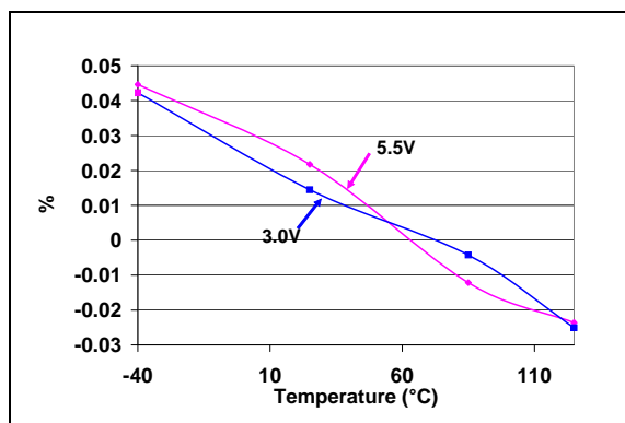
FIGURE 2-50: Resistor Network 0 to Resistor Network 1 R_{AB} (100 kΩ) Mismatch vs. V_{DD} and Temperature.
