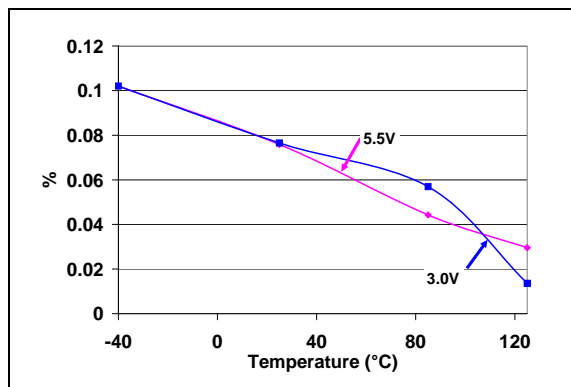
FIGURE 2-49: Resistor Network 0 to Resistor Network 1 R_{AB} (50 kΩ) Mismatch vs. V_{DD} and Temperature.
