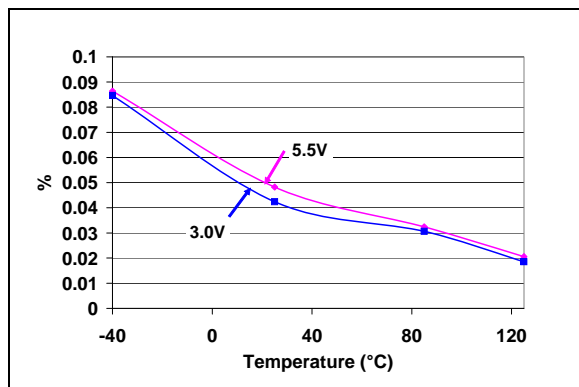
FIGURE 2-47: Resistor Network 0 to Resistor Network 1 R_{AB} (5 kΩ) Mismatch vs. V_{DD} and Temperature.
