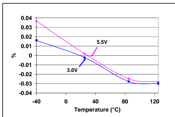
FIGURE 2-48: Resistor Network 0 to Resistor Network 1 R_{AB} (10 kΩ) Mismatch vs. V_{DD} and Temperature.
