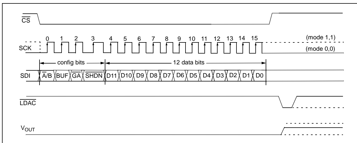
FIGURE 5-1: Write Command.
