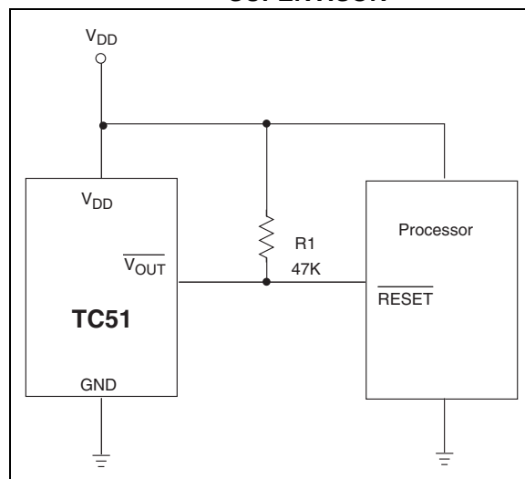
FIGURE 4-1: PROCESSOR RESET SUPERVISOR
