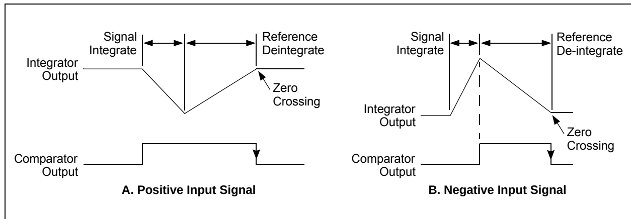
FIGURE 6-1: Comparator Output.
