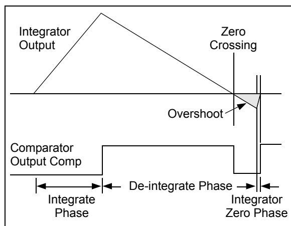
FIGURE 8-2: Overshoot.
