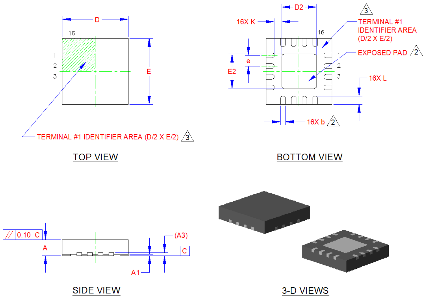
Figure 4 16-Pin QFN 4mm x 4mm Package Drawing
