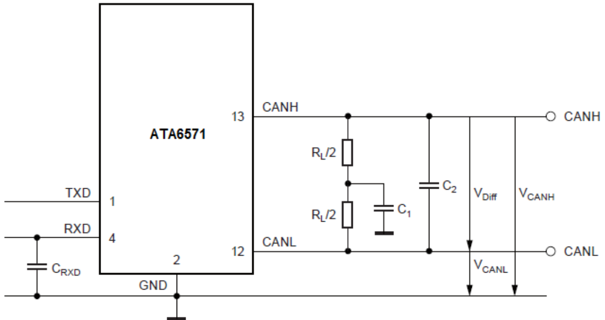
Figure 6-3. Test Circuit
