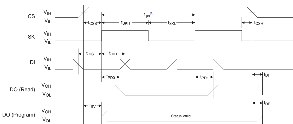
Figure 4-1. Synchronous Data Timing
