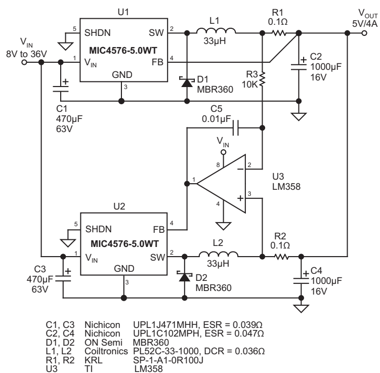
FIGURE 4-6: Parallel Switching Regulators.
