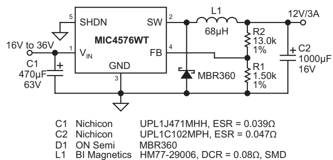
FIGURE 4-5: 16V-36V to 12V/3A Buck Converter Through Hole.
