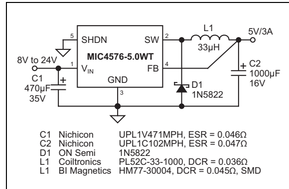
FIGURE 4-3: 8V-24V to 5V/3A Buck Converter Through Hole.
