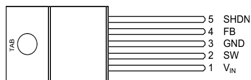
5-Pin TO-220 (T)
