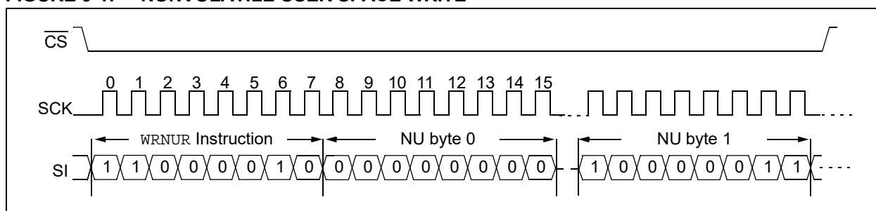
FIGURE 9-1: NONVOLATILE USER SPACE WRITE
