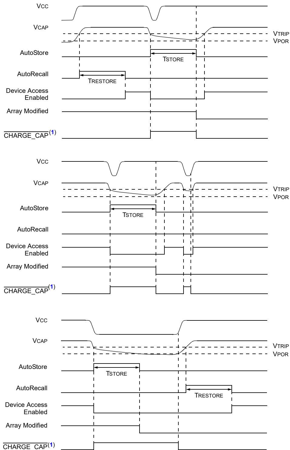
FIGURE 11-4: AUTOSTORE/AUTORECALL SCENARIOS (WITH \overline{\text{ASE}} = 0 , ARRAY MODIFIED)
