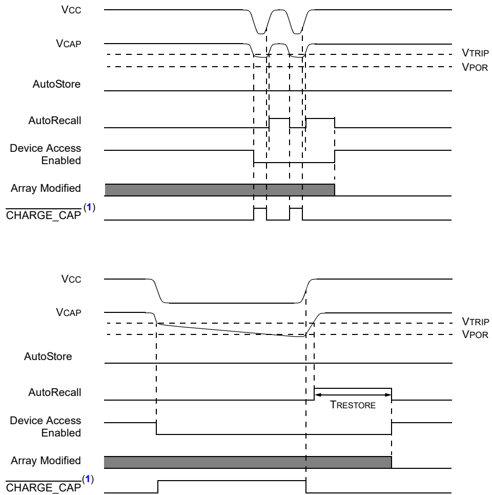
FIGURE 11-5: AUTOSTORE/AUTORECALL SCENARIOS (WITH \overline{\text{ASE}} = 1 OR ARRAY NOT MODIFIED)
