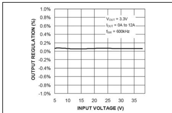
FIGURE 2-21: Output Regulation vs. Input Voltage (MIC2102).
