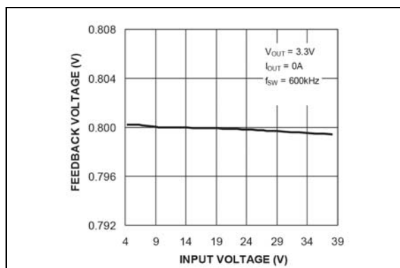
FIGURE 2-20: Feedback Voltage vs. Input Voltage (MIC2102).
