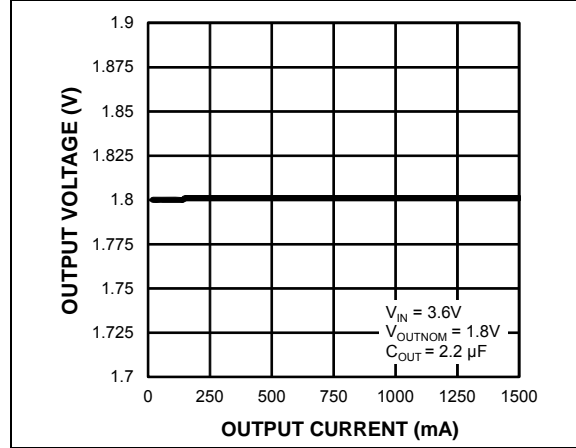
FIGURE 2-11: Load Regulation.
