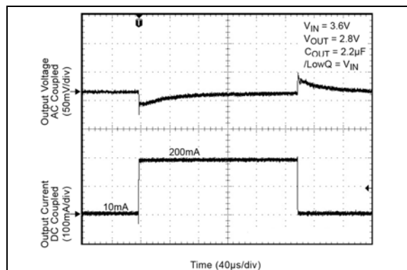
FIGURE 2-24: LDO2 (Normal Mode) Load Transient.
