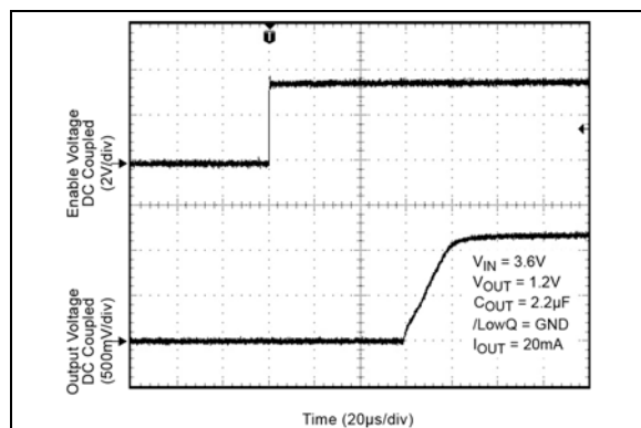
FIGURE 2-26: DC/DC (LOWQ Mode) Start-Up Waveform.
