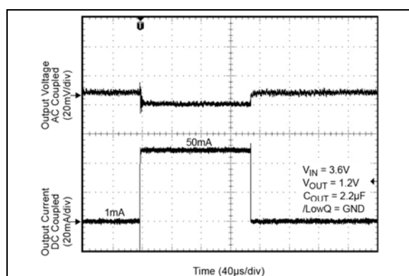
FIGURE 2-25: DC/DC (LOWQ Mode) Load Transient.
