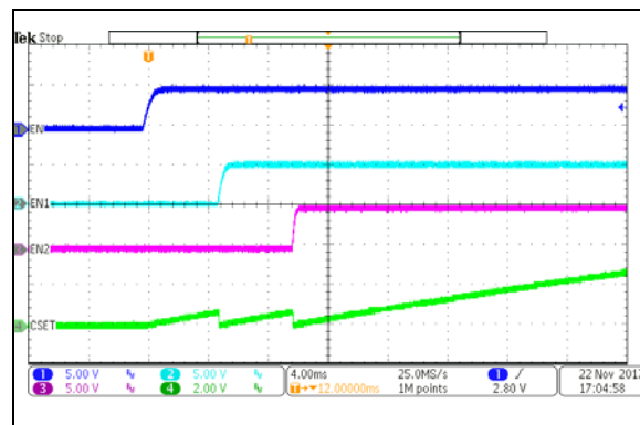
FIGURE 2-33: CSET Pin Voltage for Correct Sequencing.
