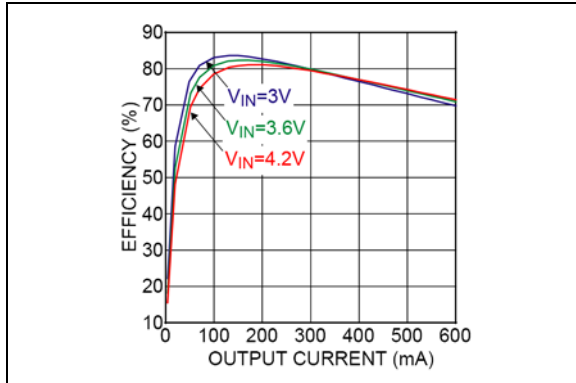
FIGURE 2-1: 1.2V_{\text{OUT}} Efficiency.
