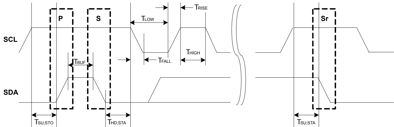
Figure 30-7. SCL Timing
